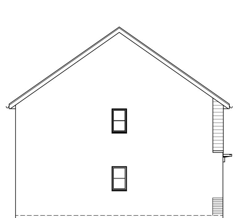
Side Elevation
