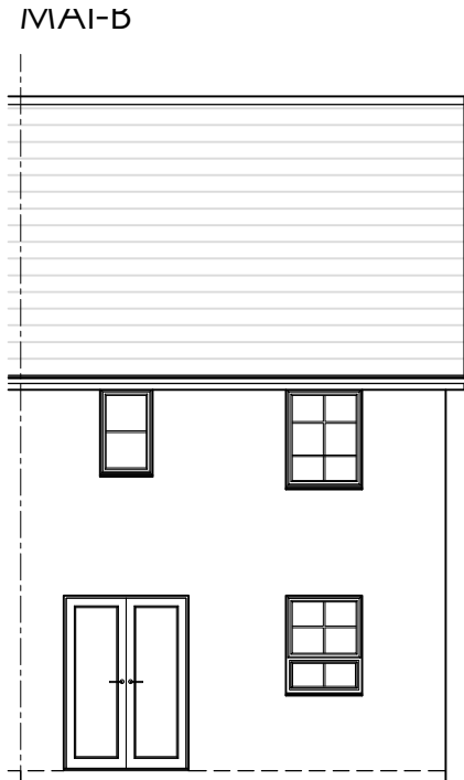
Rear Elevation
