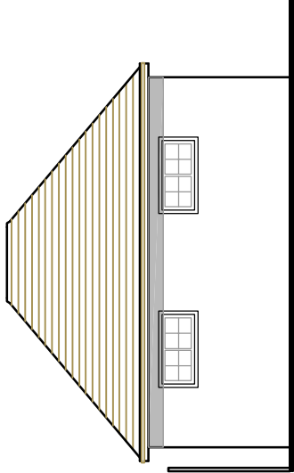
NORTH ELEVATION 1:100
