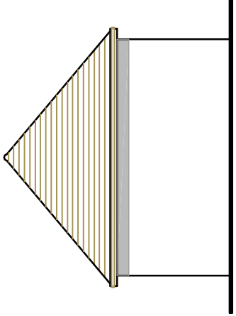
EAST ELEVATION 1:100
