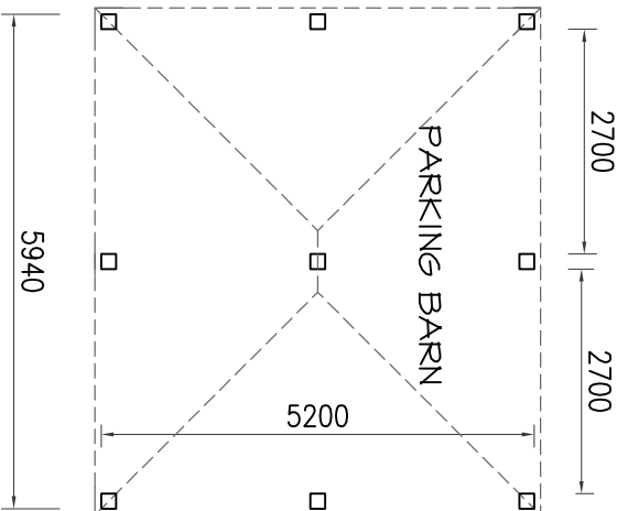
CAR BARN - PLAN VIEW PLOTS 4 & 5
