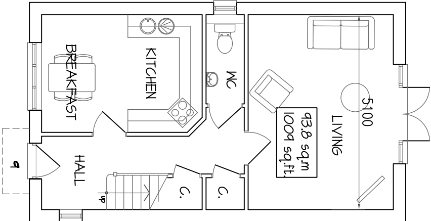
GROUND FLOOR 3 BEDROOM
