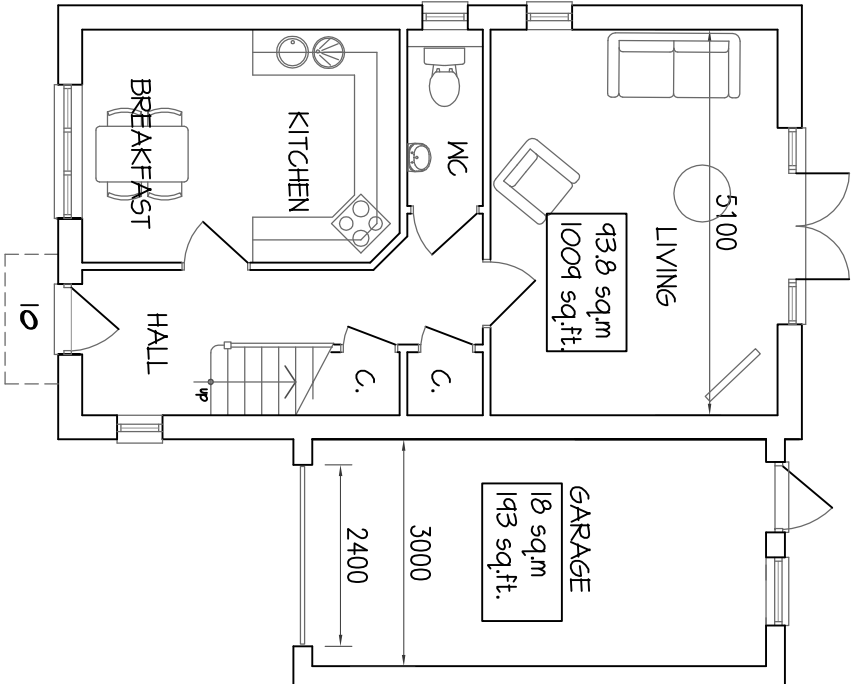
GROUND FLOOR 3 BEDROOM
