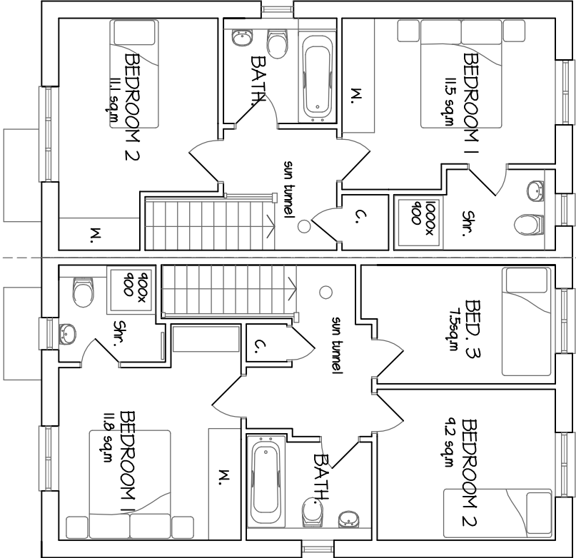
FIRST FLOOR
