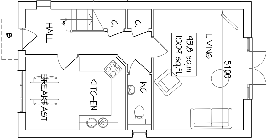
GROUND FLOOR 3 BEDROOM
