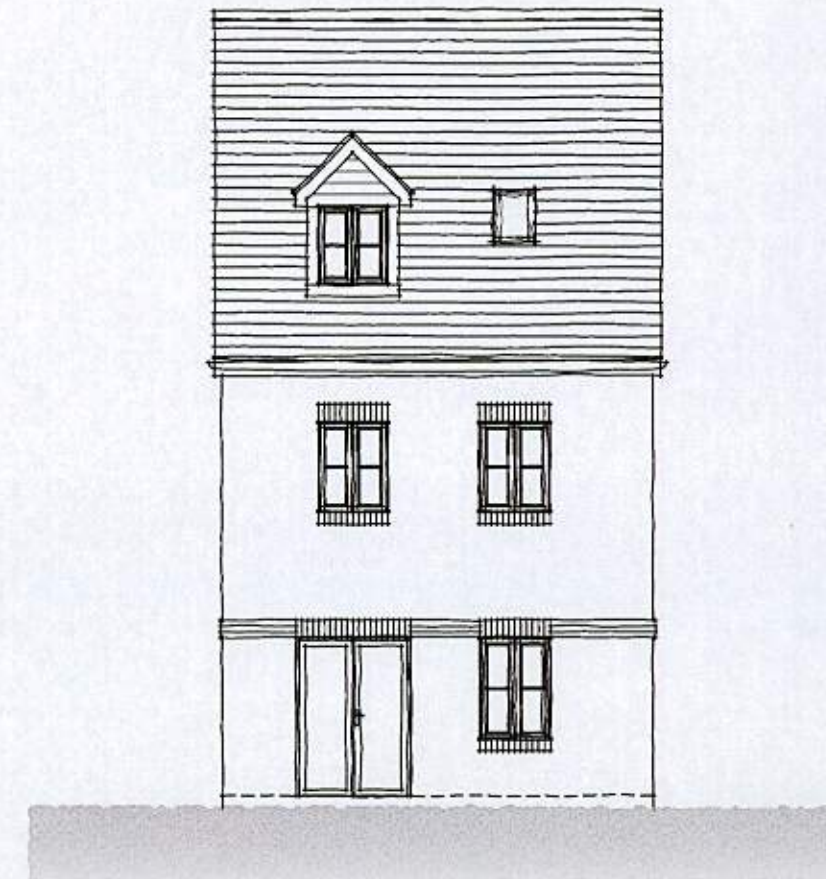
REAR ELEVATION
