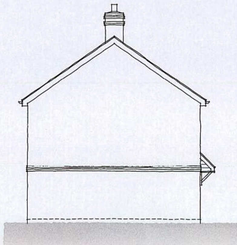
SIDE ELEVATION
