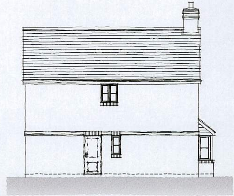
REAR ELEVATION
