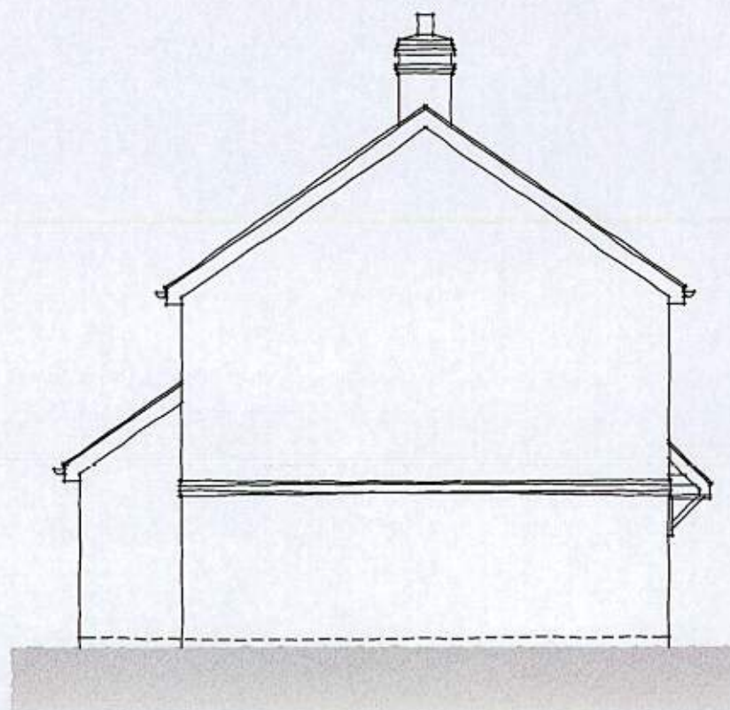
SIDE ELEVATION
