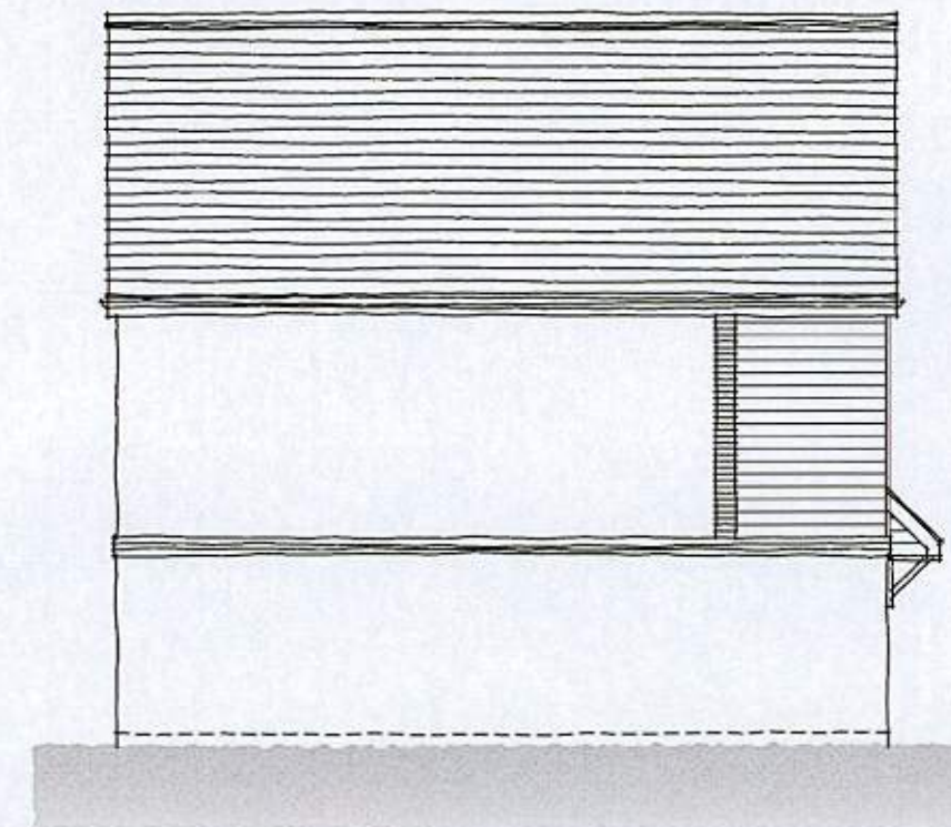
SIDE ELEVATION
