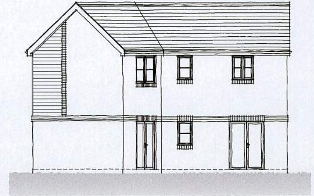
REAR ELEVATION
