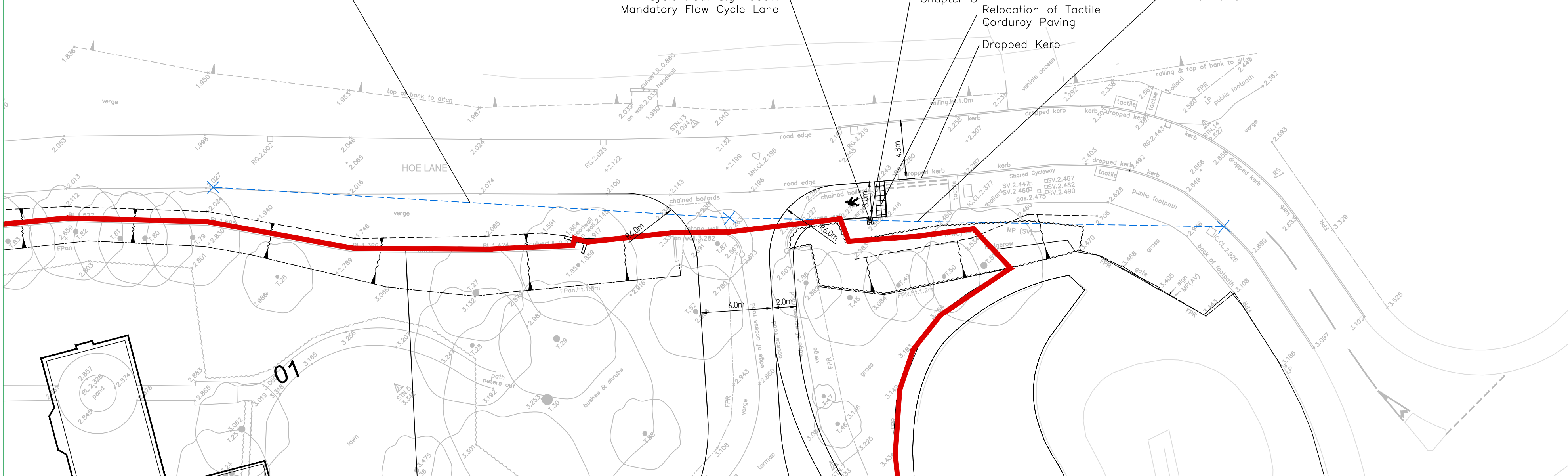
Refuse Vehicle Egress Scale 1:250
