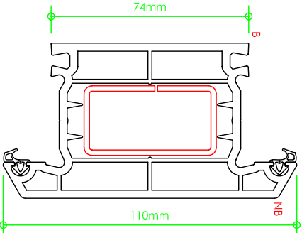
10mm Z door sash 2mm box reinforcement -102141 -113222
