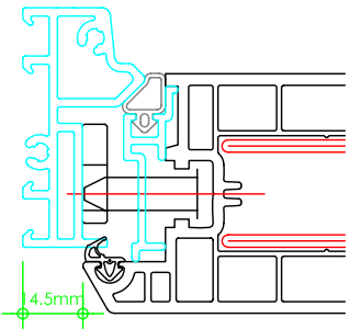
29mm aluminium low threshold aluminium gasket corner 27mm low threshold keep plate threshold gasket -104186 -104159 -141126 -112112
