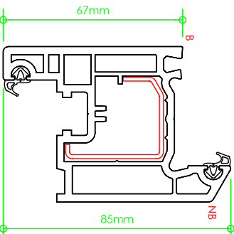
85mm III/Turn & door sash reinforcement -103169 -113225
