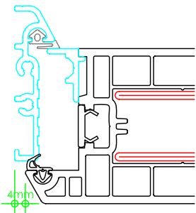
15mm aluminium low threshold 15mm aluminium sealing strip threshold gasket -104215 -104214 -112135
