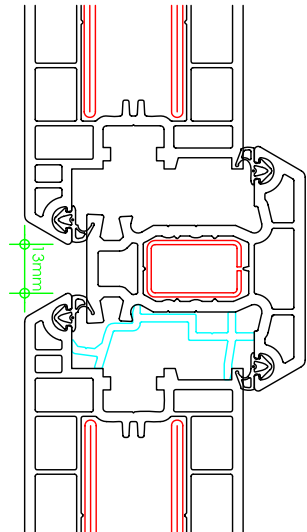
aluminium french door coupling -104249
