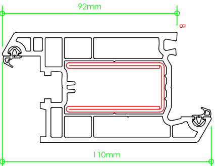
10mm Z door sash piped reinforcement 2mm box reinforcement u channel reinforcement -105128 -113223 -113223 -113282
