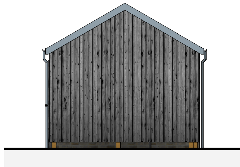
Side Elevation 1
