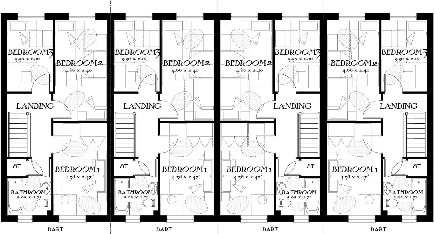
First Floor
