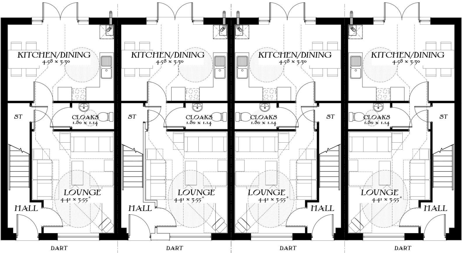
Ground Floor
