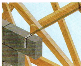
Anchorage of gable end to roof-structure, M305
