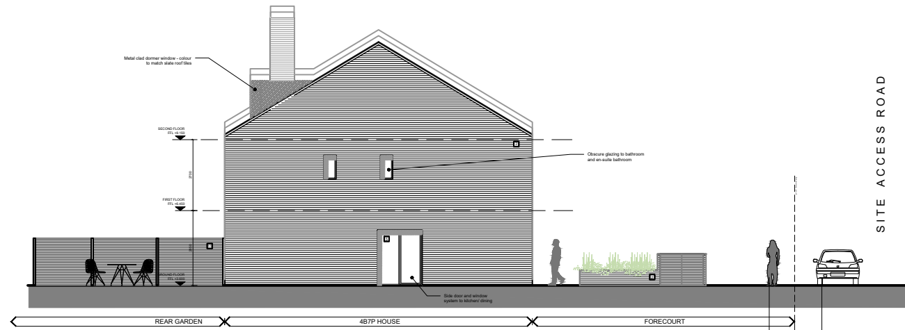
4-4 side elevation
