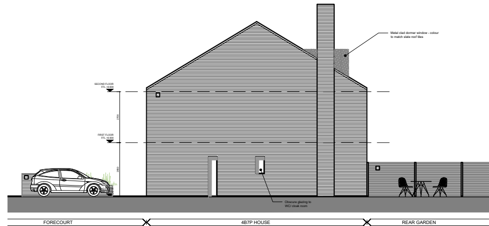
2-2 side elevation
