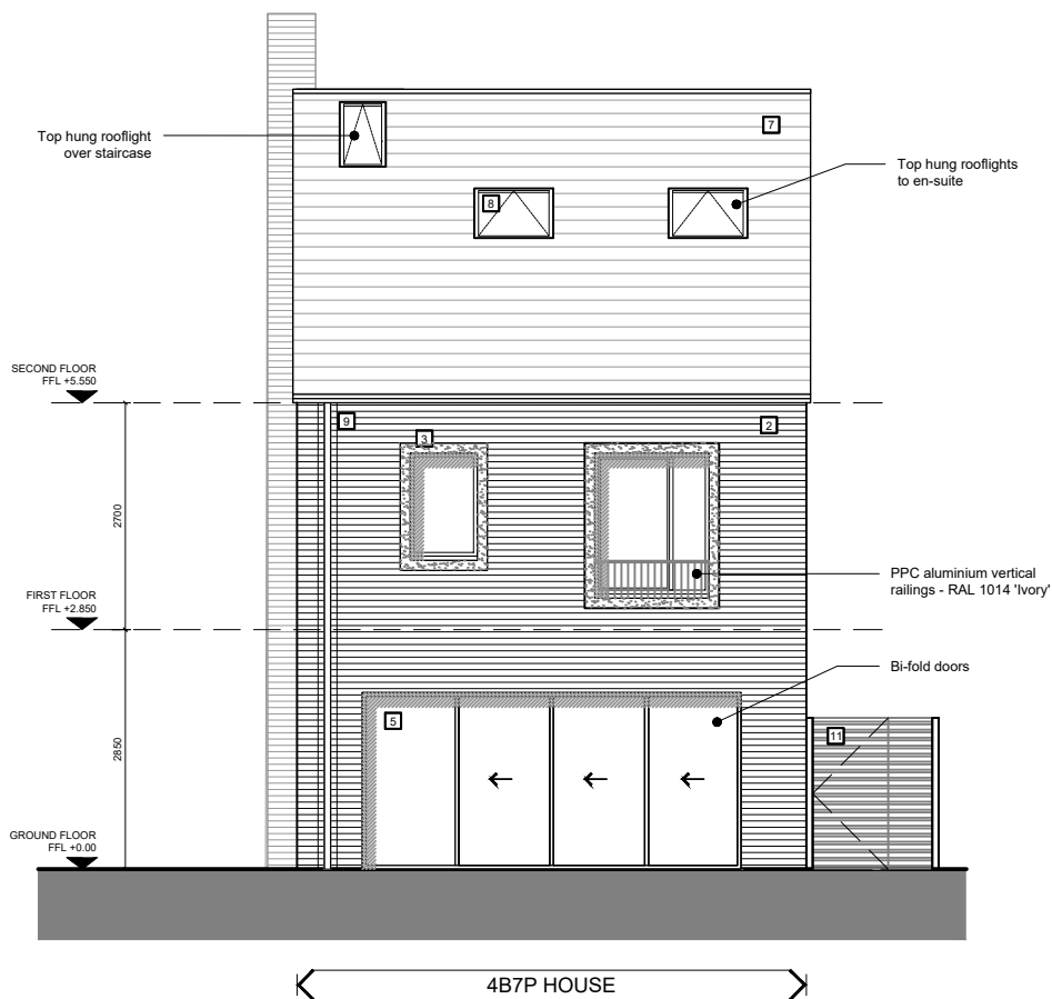
2-2 rear elevation
