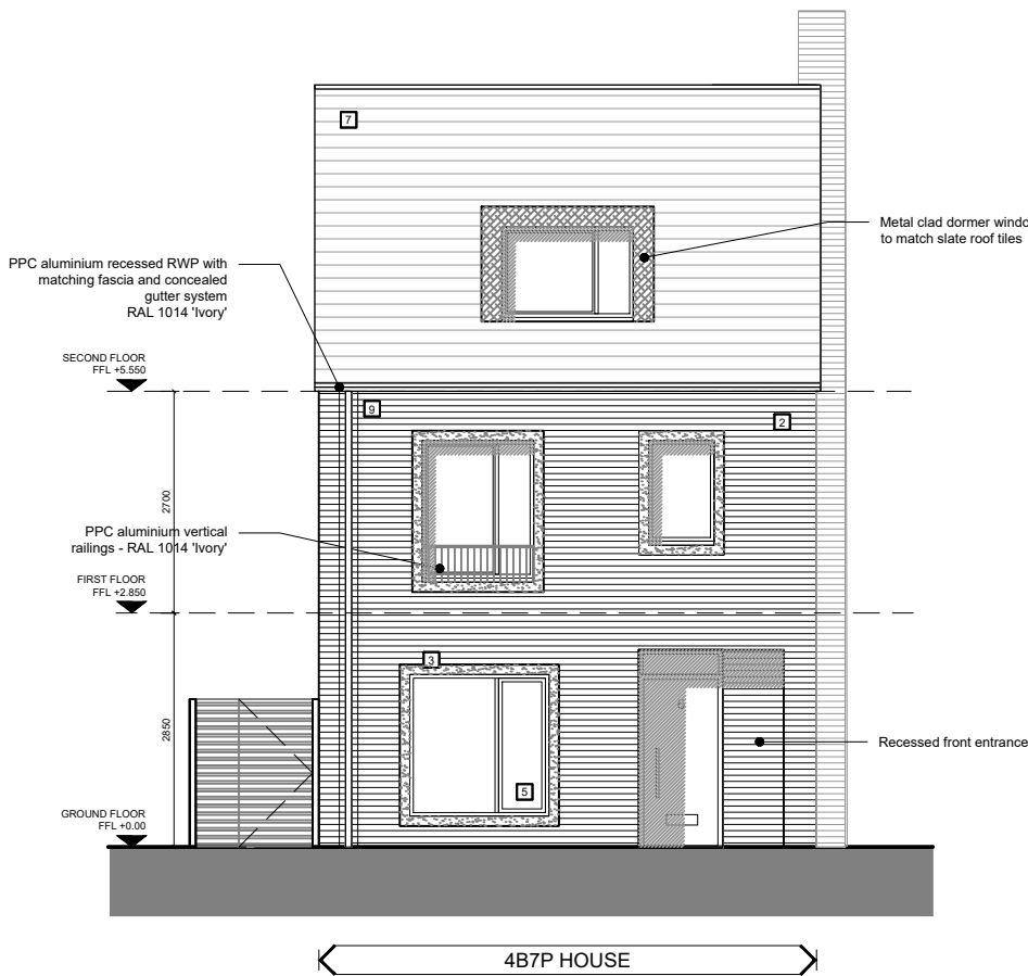
1-1 front elevation
