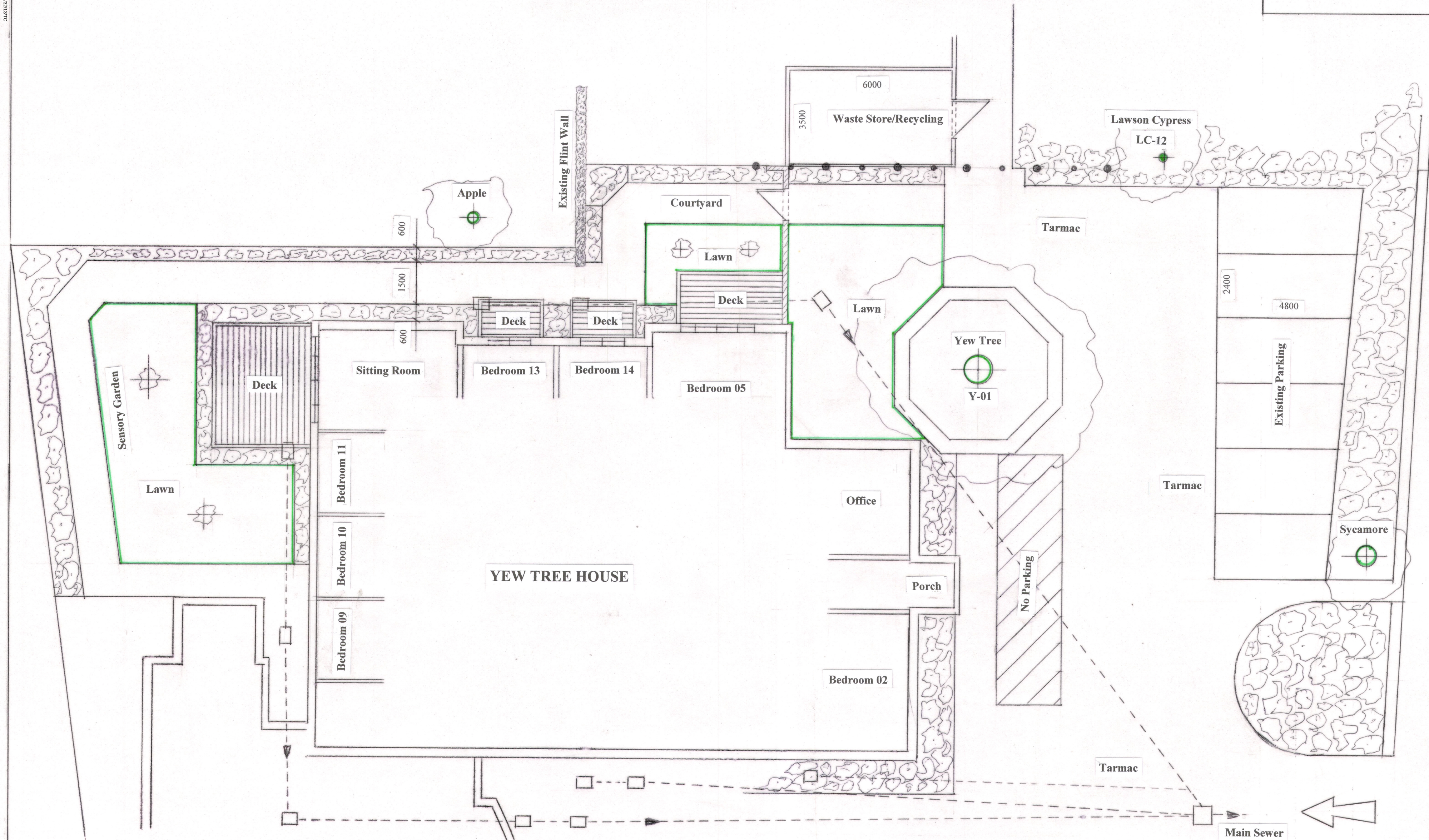
PROPOSED LANDSCAPE PLAN 1:100
