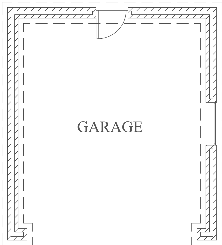
GARAGE FOUNDATION LAYOUT
