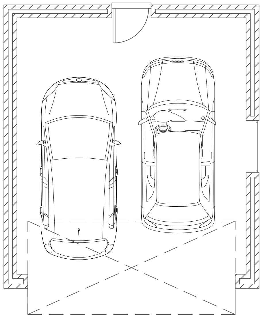
GARAGE GENERAL LAYOUT
