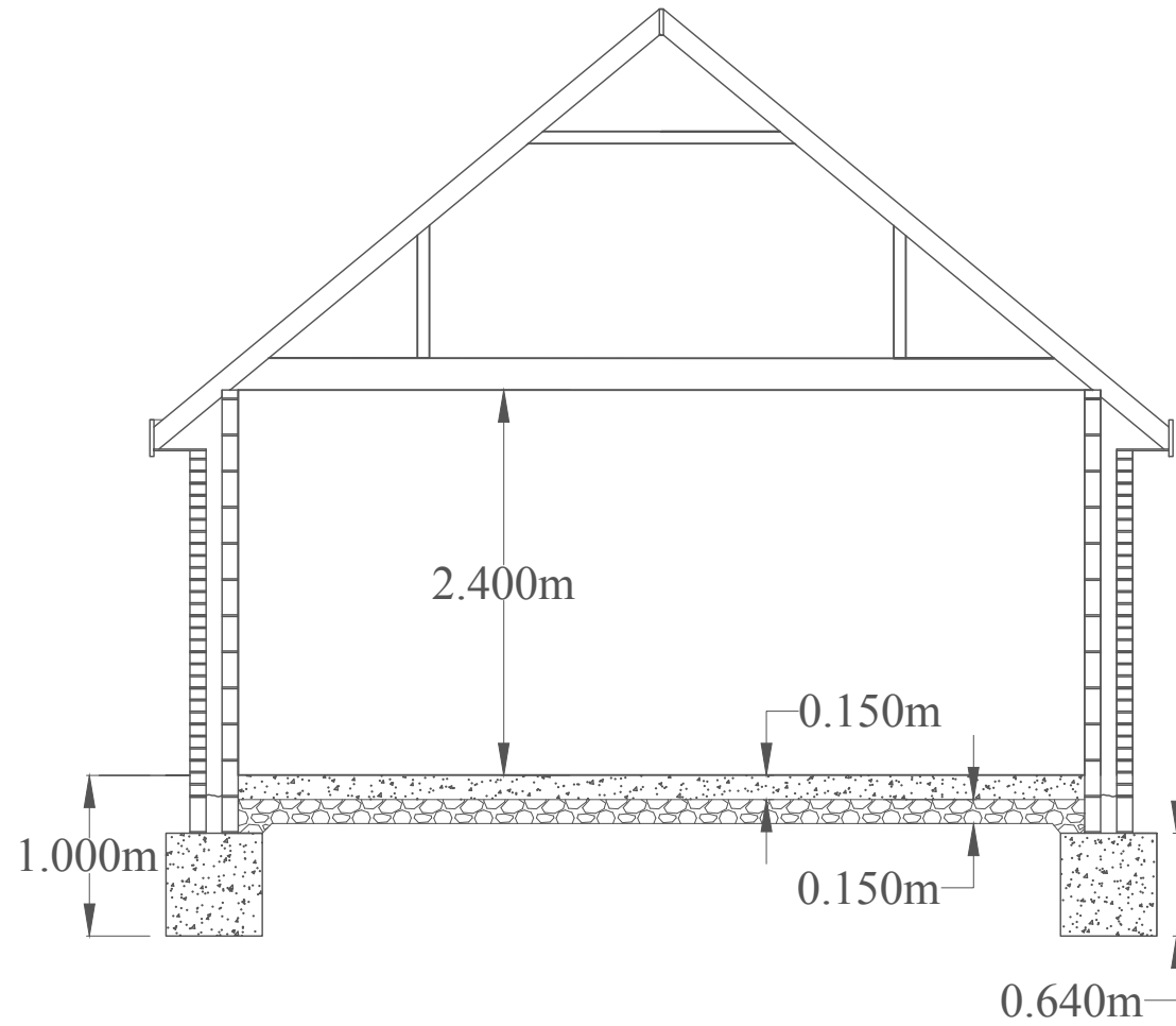
GARAGE FRONT SECTION
