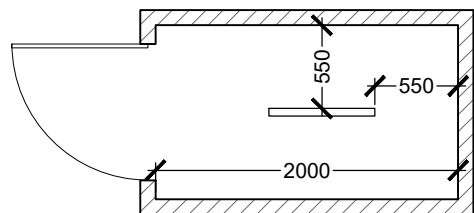
Proposed Floor Plan 1:50
