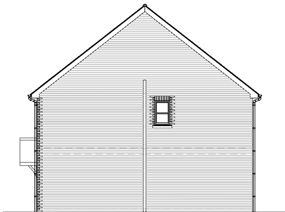
West Elevation
