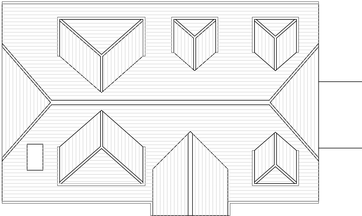
Proposed - Roof plan scale 1.100 @ A3
