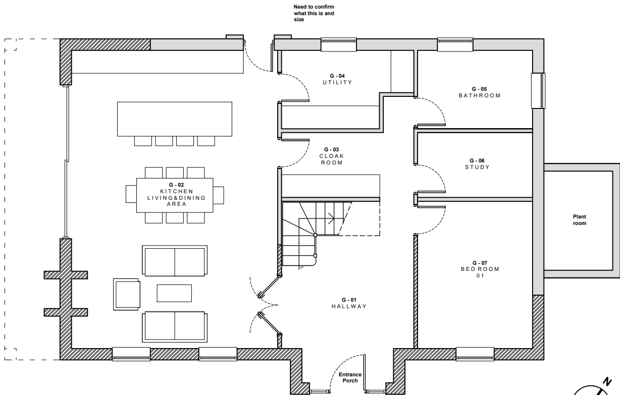
Proposed - Ground Floor Plan scale 1.100 @ A3
