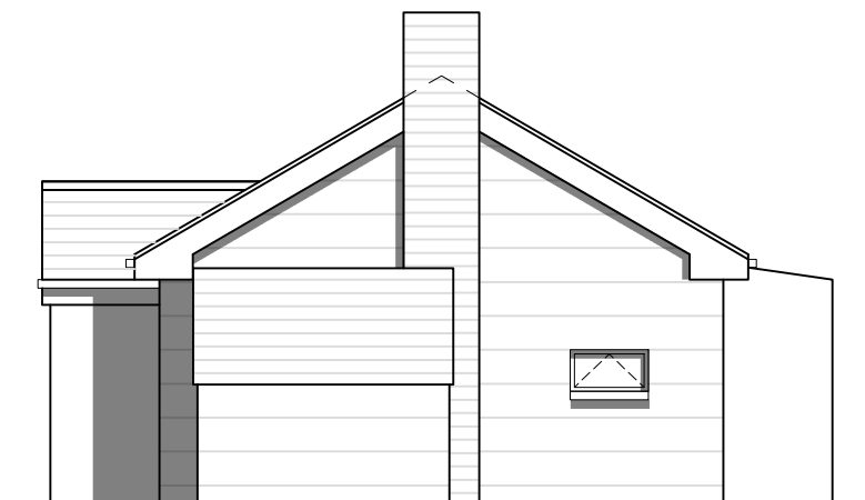
Existing - Elevation North East scale 1.100 @ A3
