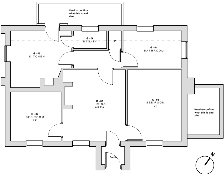
Existing - Ground floor layout scale 1.100 @ A3
