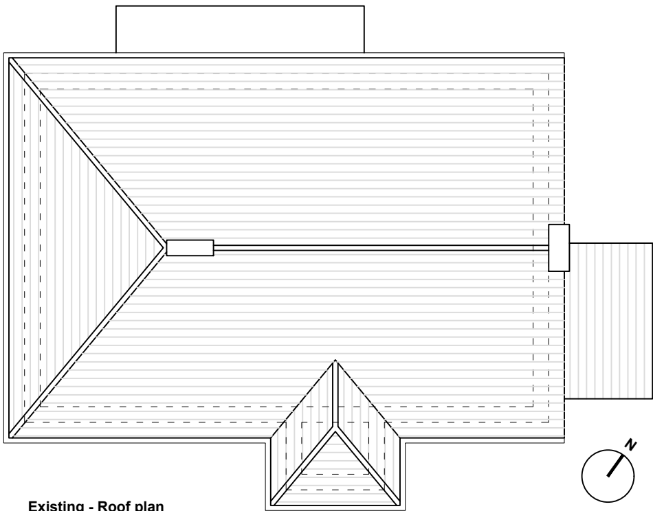
Existing - Roof plan scale 1.100 @ A3
