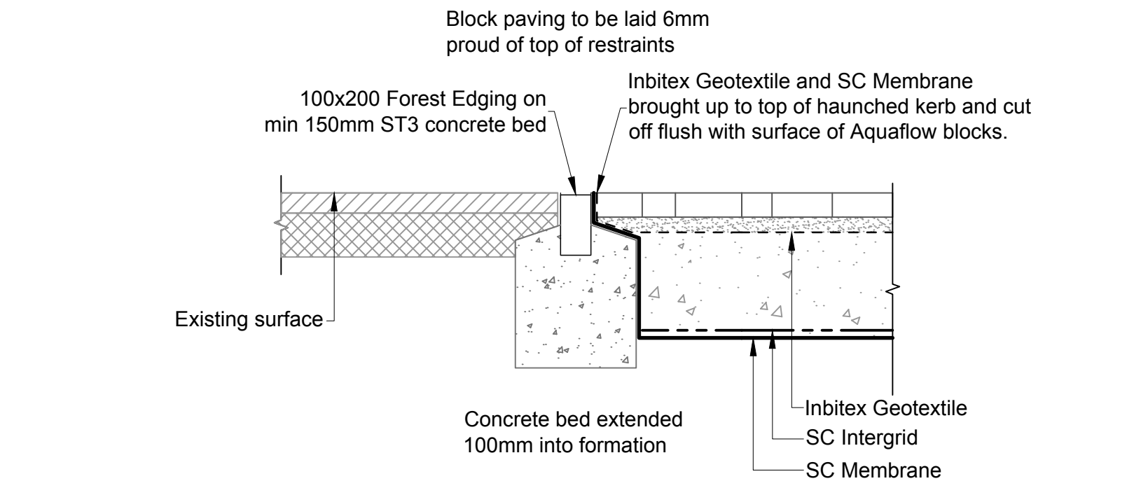
FULL HEIGHT RESTRAINT DETAIL (EXISTING CONSTRUCTION TO FORMPAVE AQUAFLOW TRANSITION)
