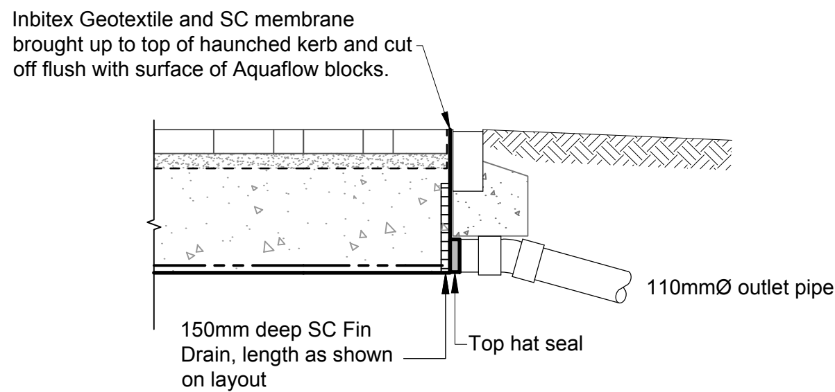
TYPICAL FIN DRAIN OUTLET DETAIL
