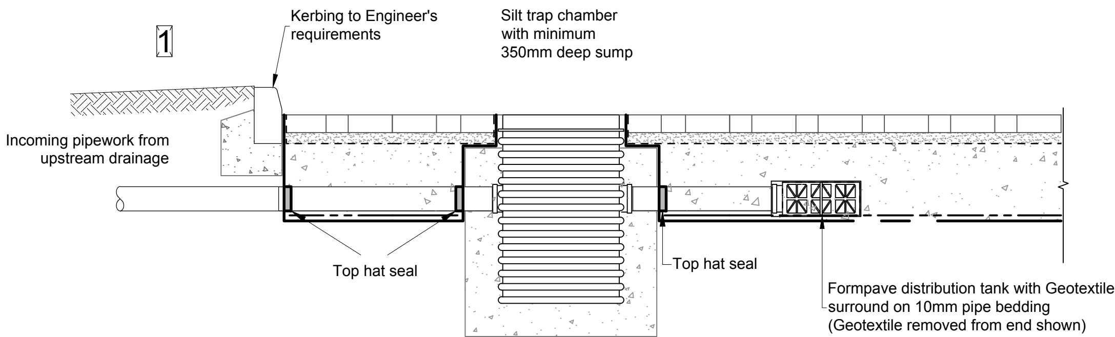
TYPICAL INLET DETAIL (SINGLE SIZE 0.35 x 0.70 x 0.15m DEEP)
