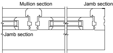
Window Section B-B
