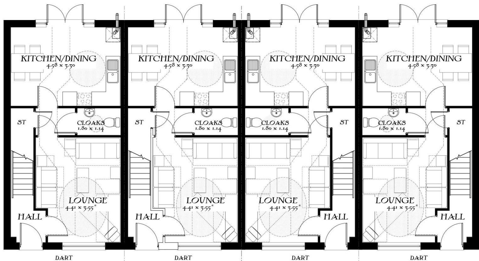
Ground Floor
