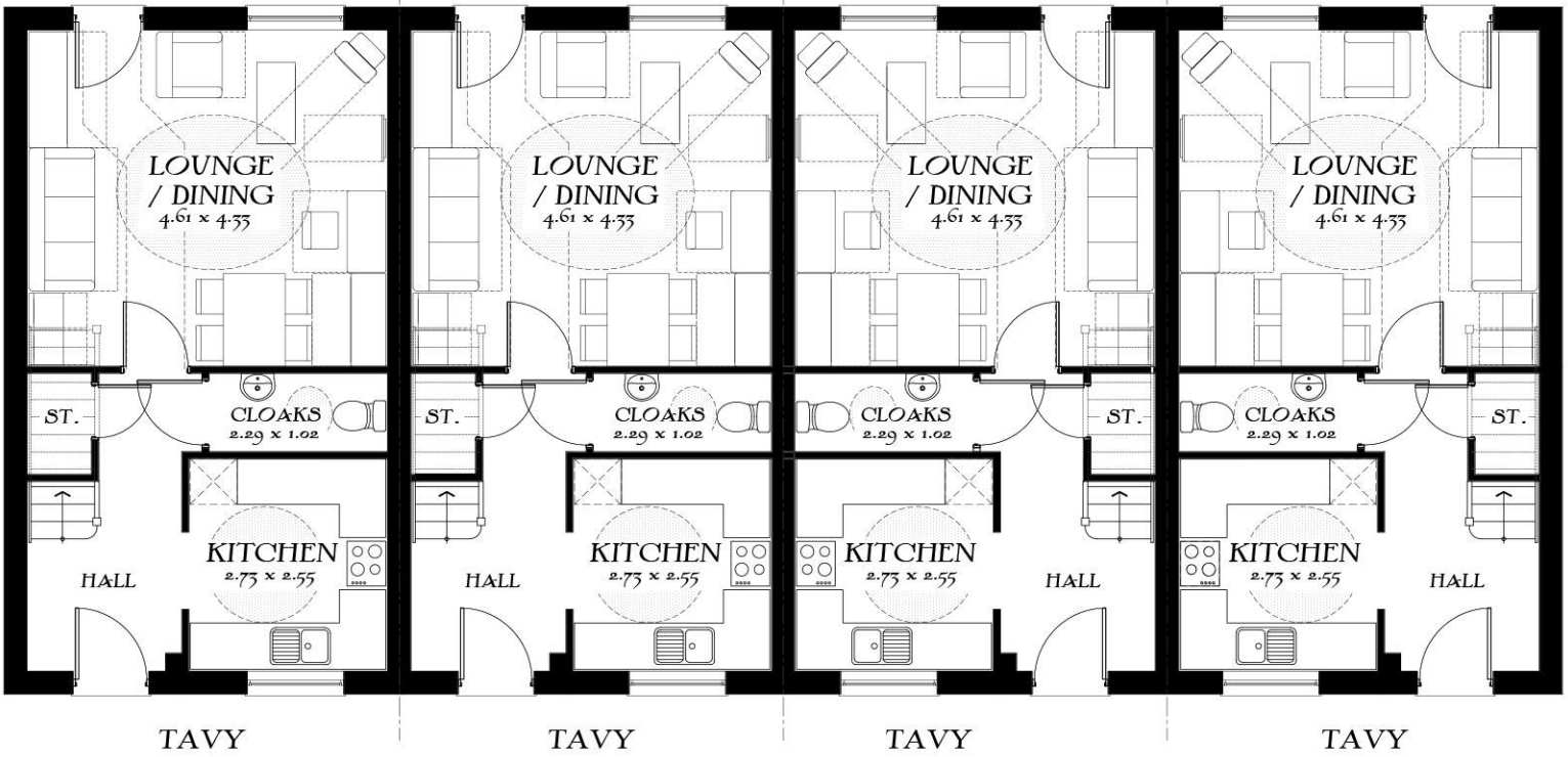
Ground Floor
