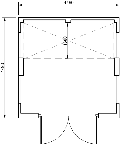
Floor Plan
