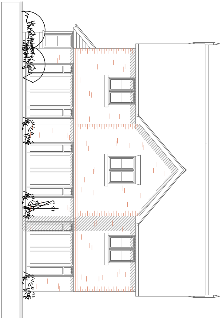
REAR ELEVATION - South
