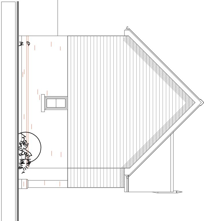
SIDE ELEVATION - East
