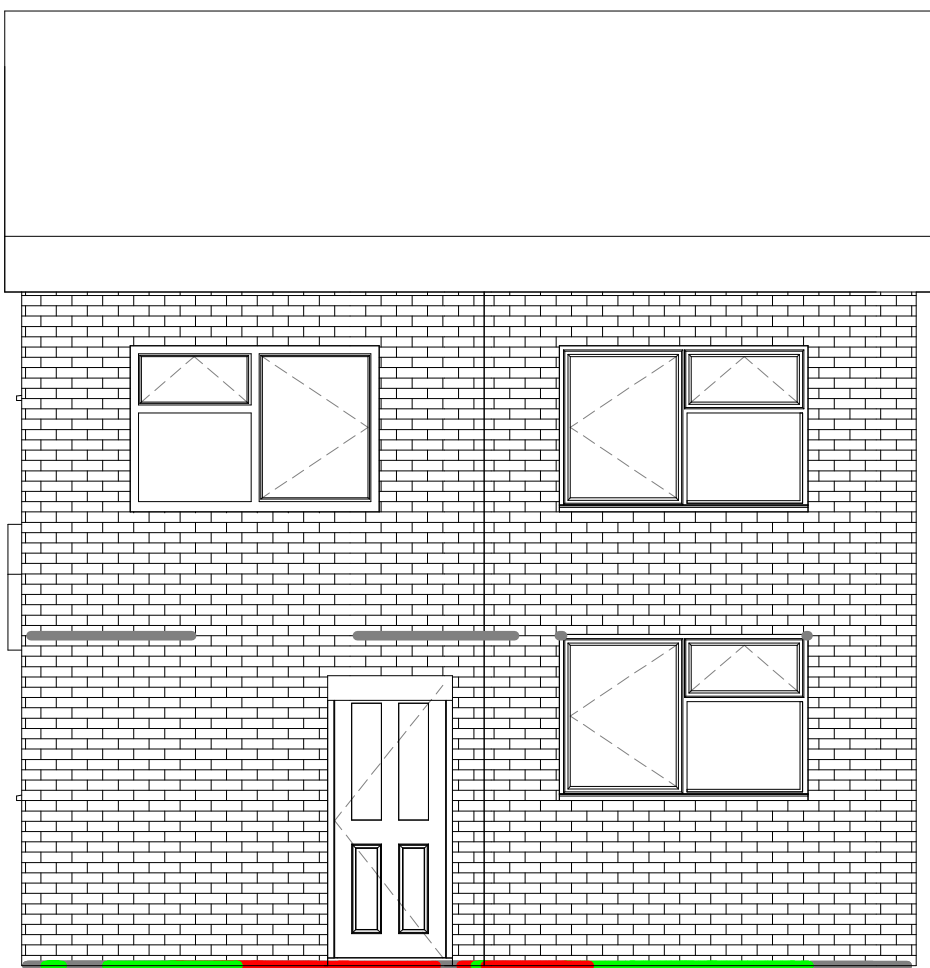
3 South - Dependent 1 1 : 50
