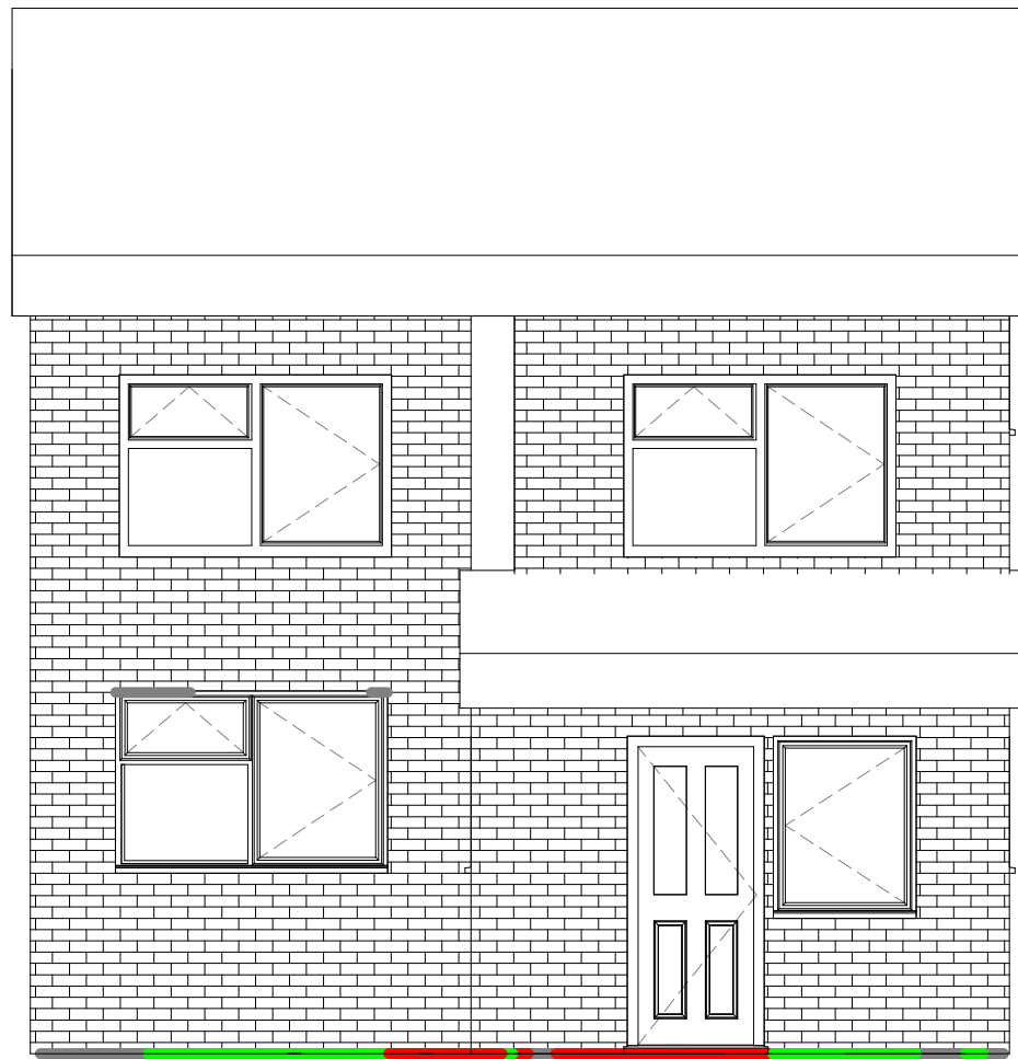
2 North - Dependent 1 1 : 50
