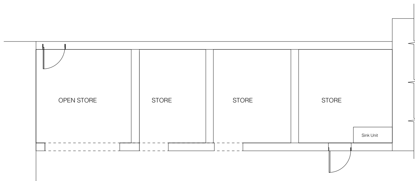
EXISTING FLOOR PLAN - W SECTION
