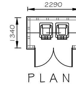
BIN STORES FOR BARN 1, 2 & 3
