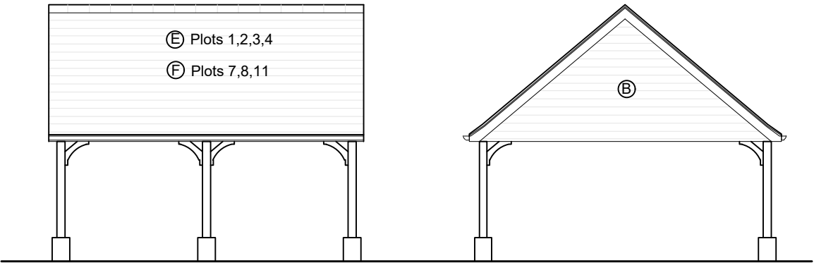
FRONT/REAR elevation
