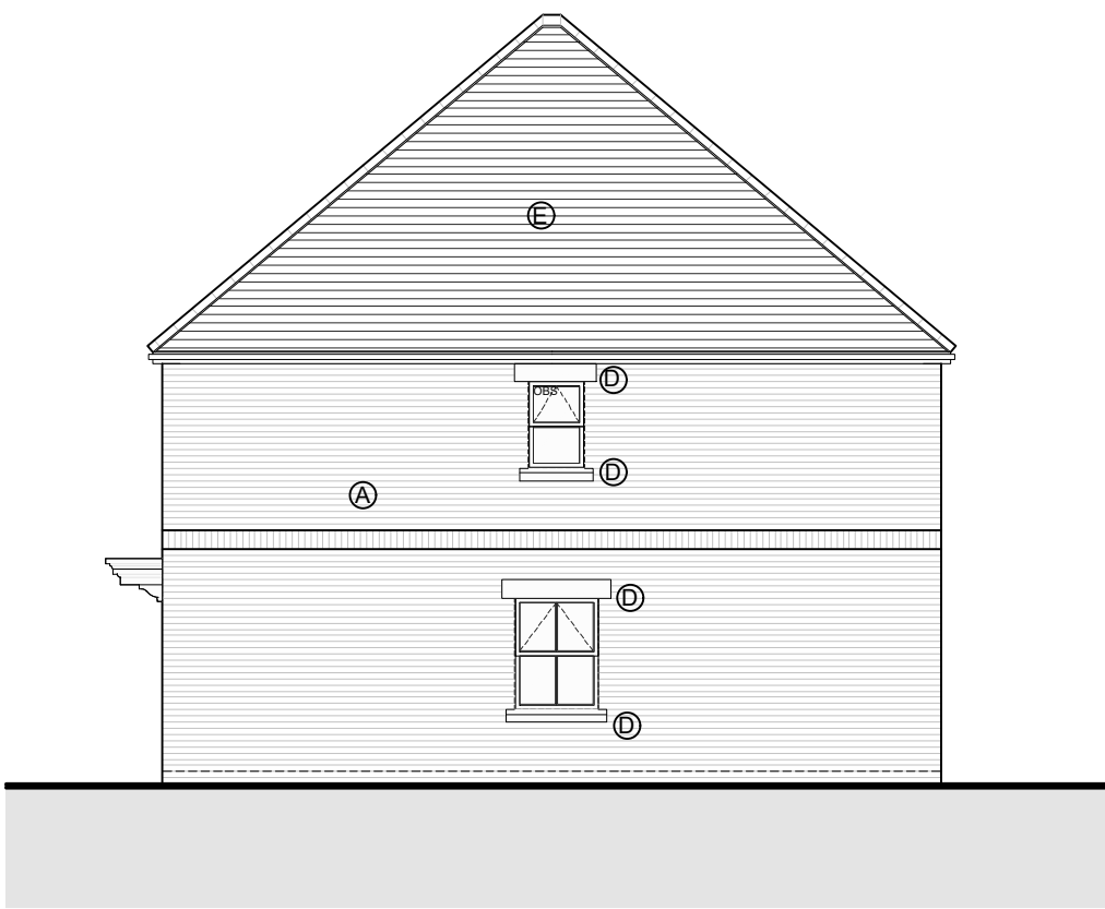
SIDE elevation
