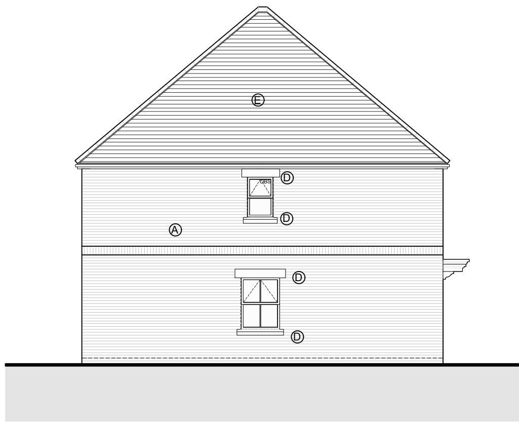
SIDE elevation
