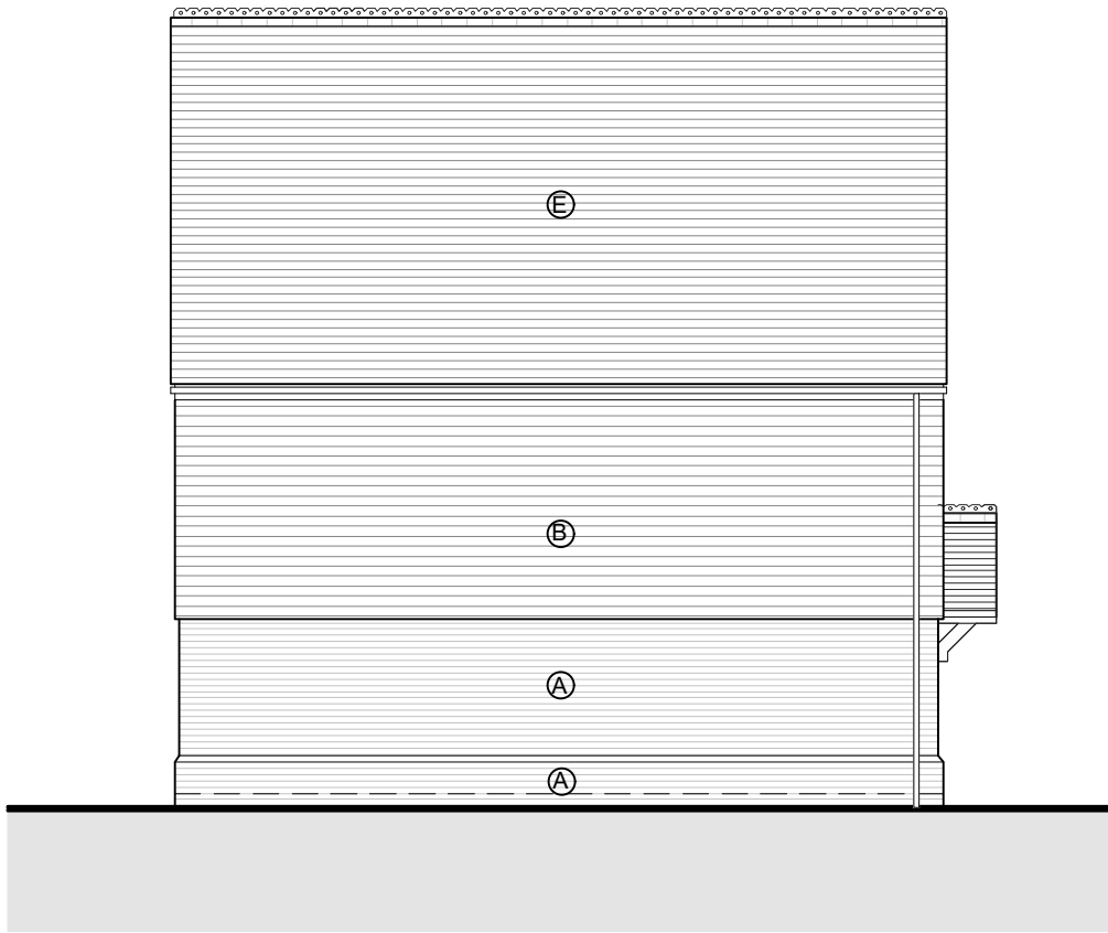
SIDE elevation
