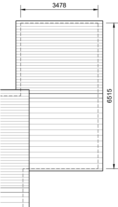
Roof Plan
