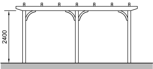
Front Elevation
