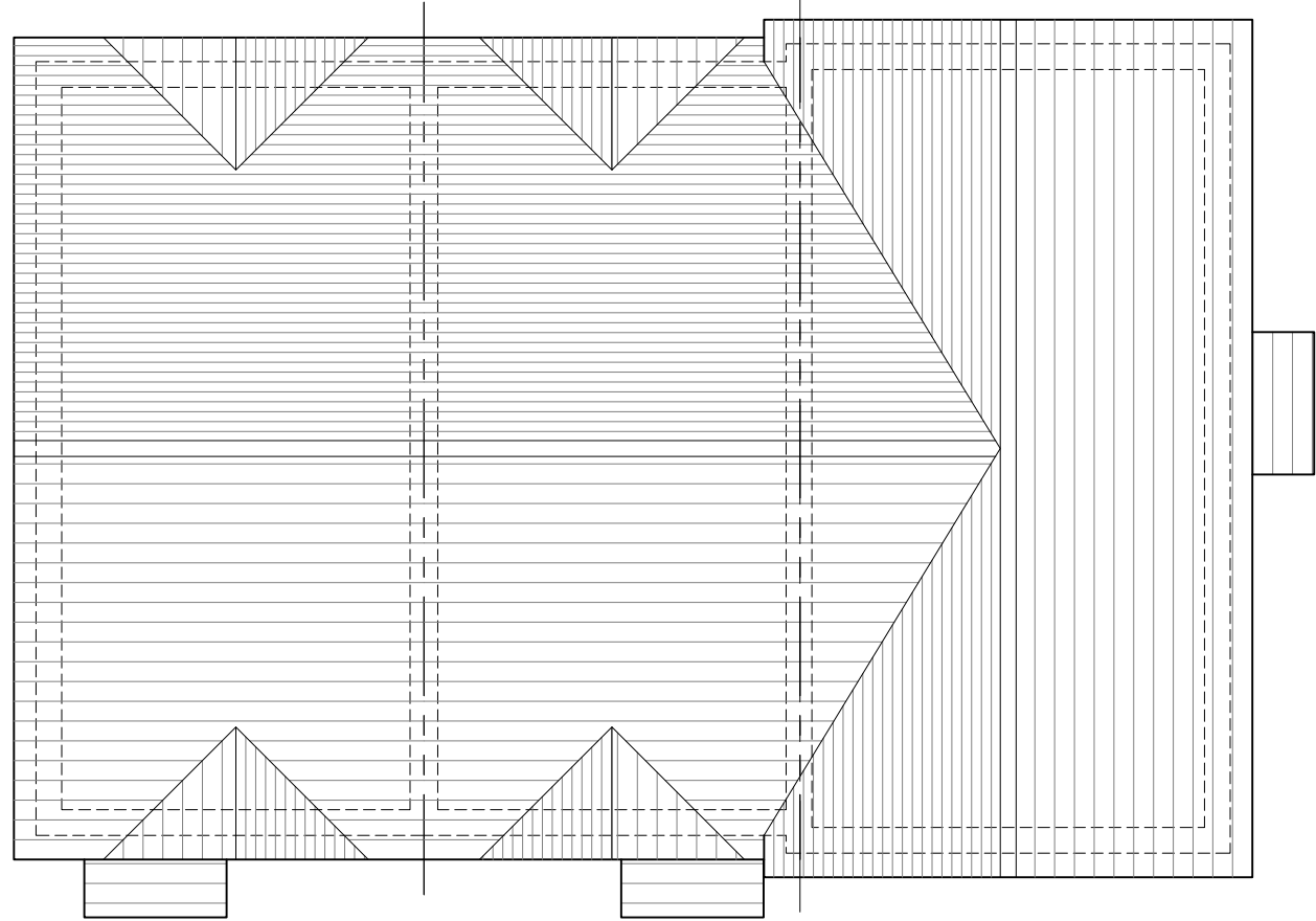
Roof Plan
