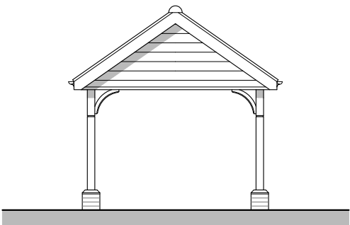
Rear Elevation
