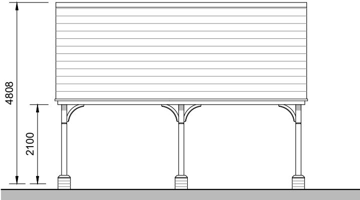
Side Elevation B
