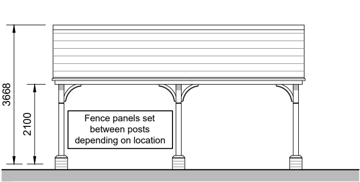
Side Elevation A
