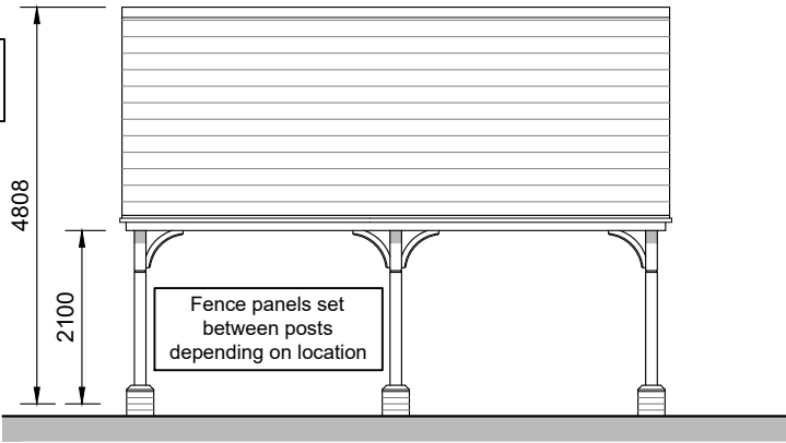
Side Elevation A
