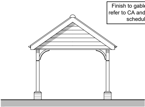
Front Elevation
