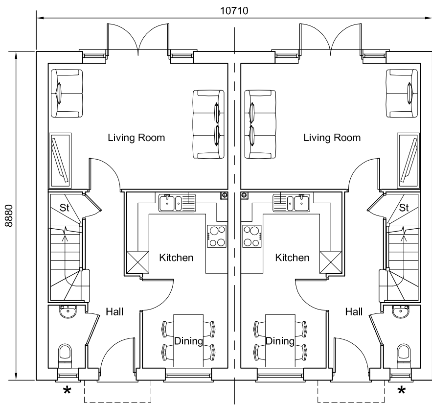
Ground Floor Plan ★ - Obscured glazing
