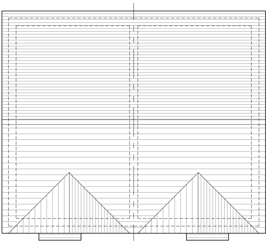
Roof Plan Plots : 129/130, 131/132,
