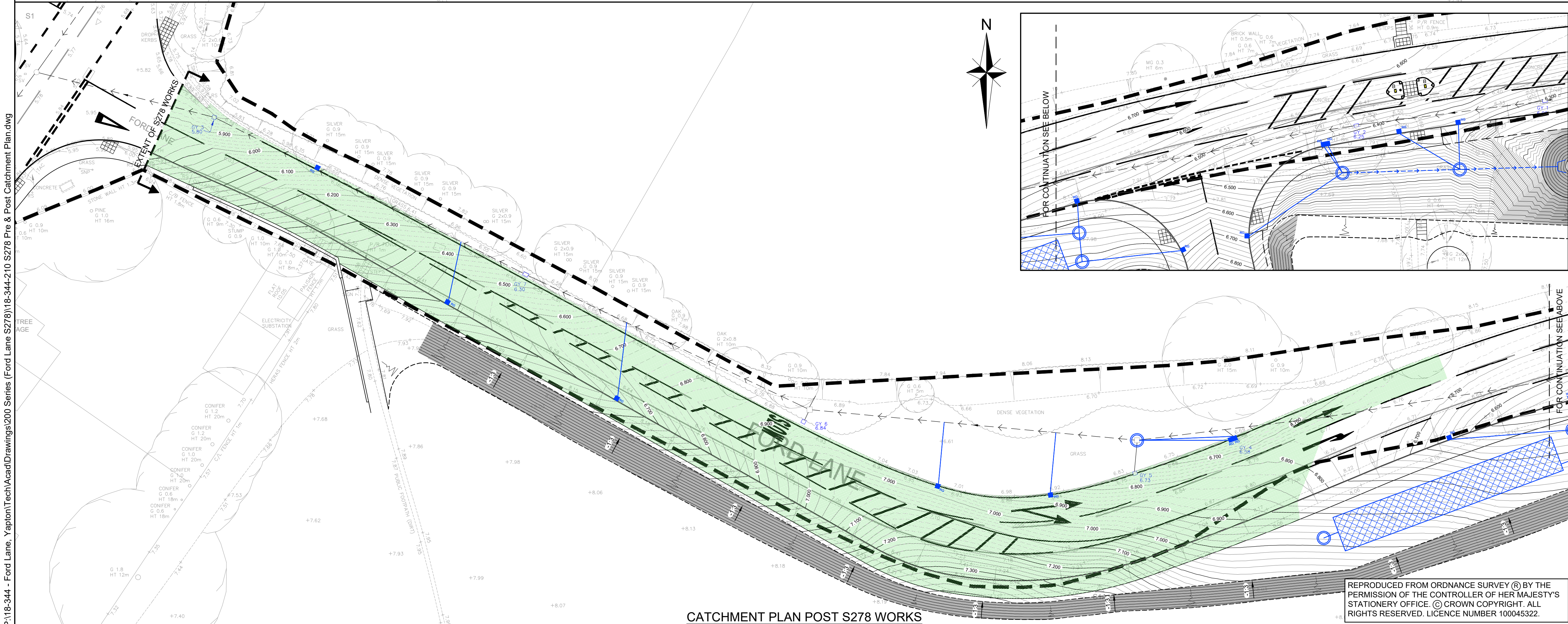
CATCHMENT PLAN POST S278 WORKS
