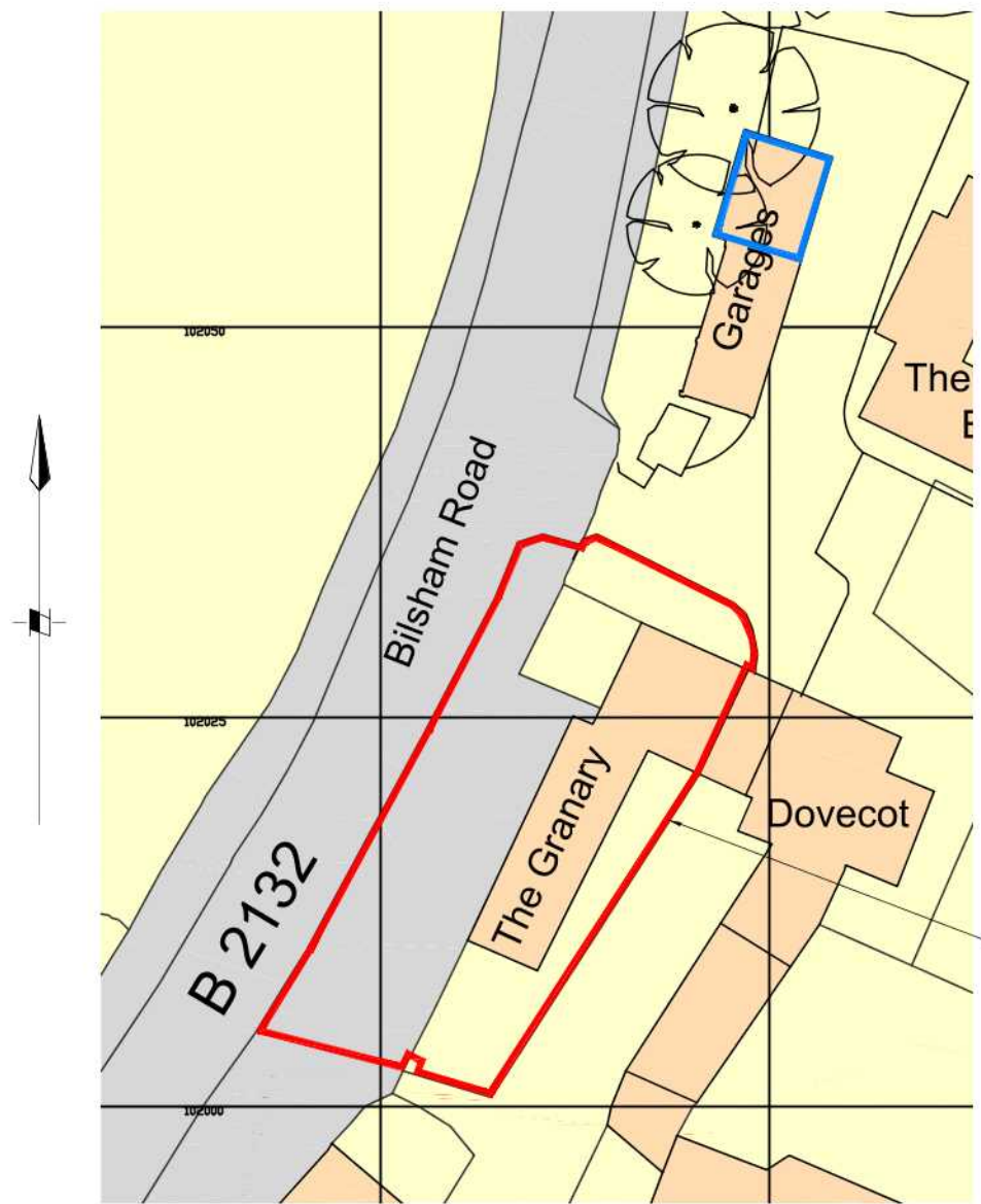
Site / Block plan 1:500 @ A3
