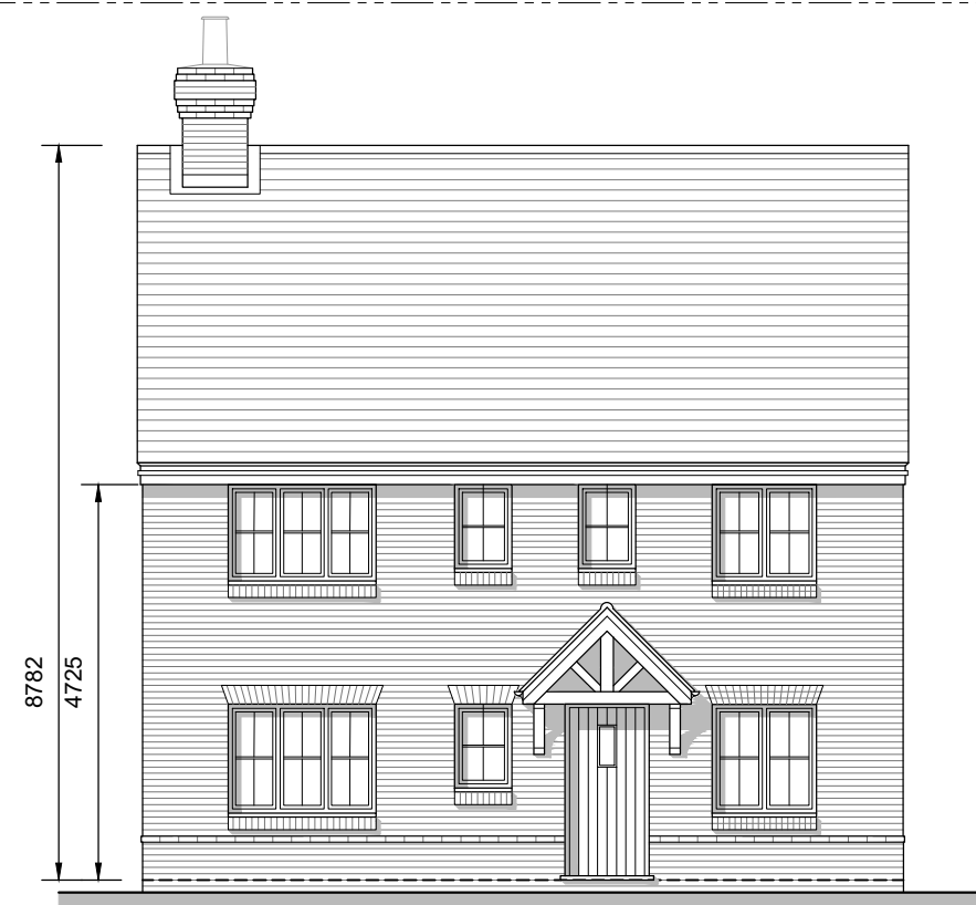
Front Elevation
