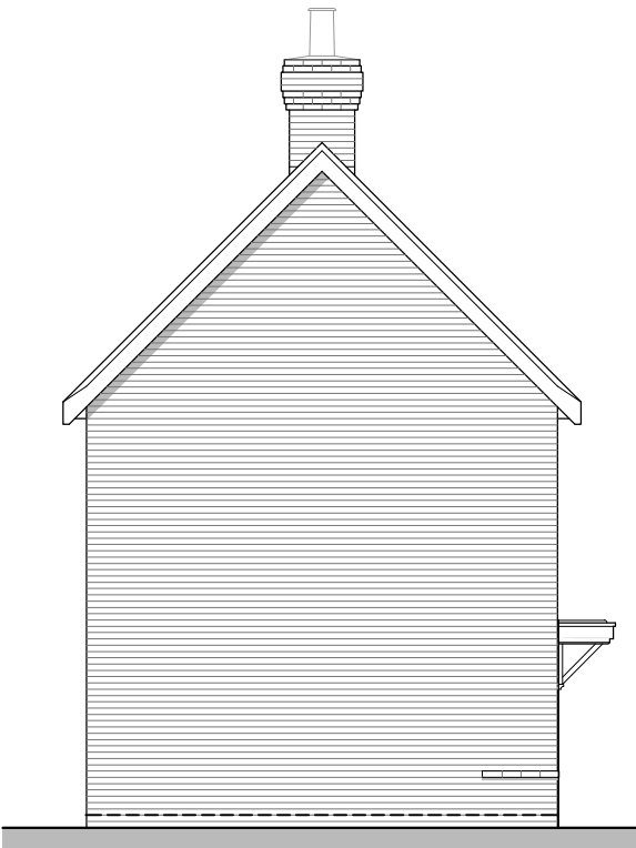
Side Elevation A
