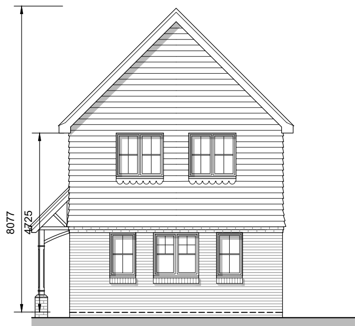
Front Elevation
