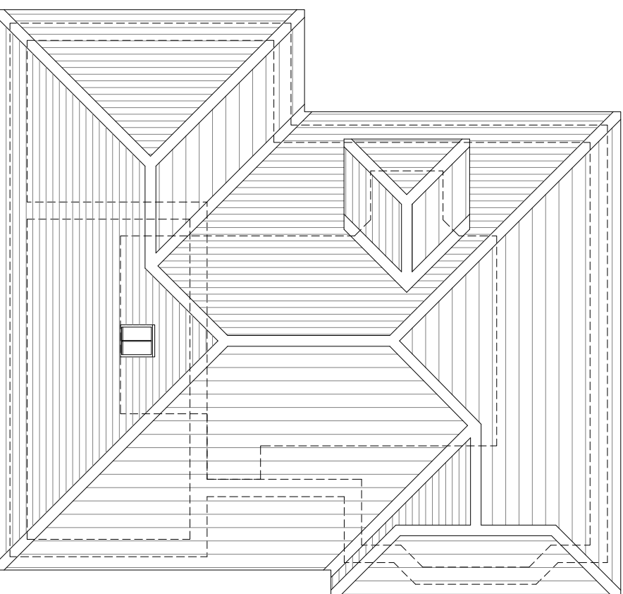
Roof Plan
