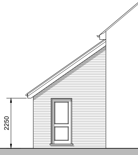
Side Elevation A
