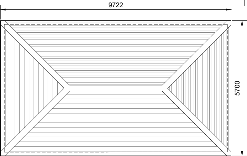
Roof Plan
