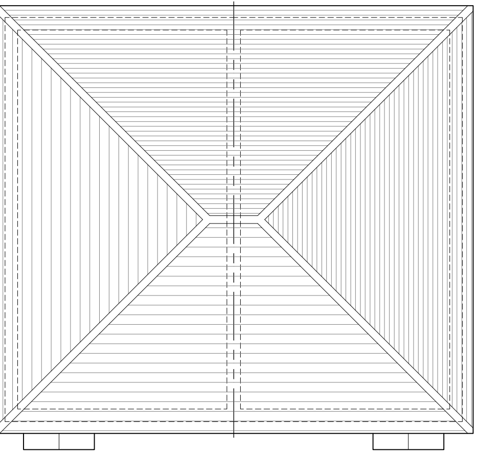
Roof Plan
