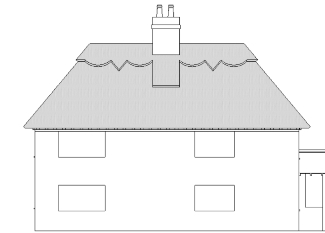
EXISTING NORTH ELEVATION 1:100
