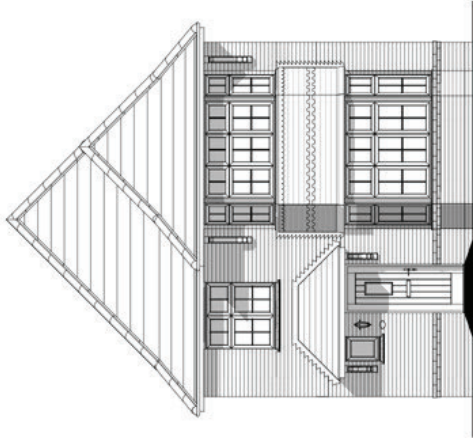
Front Elevation
